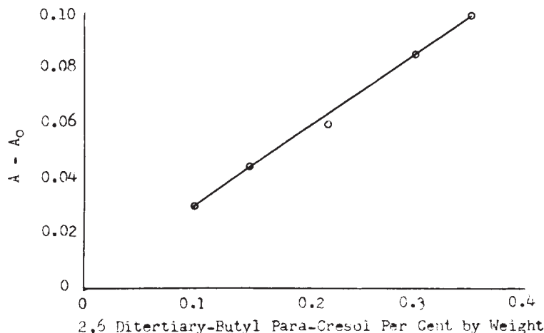
FIG. 2 Calibration Curve for Determining the Percent by Weight of 2,6-Ditertiary-Butyl Paracresol in Electrical Insulating Oil
