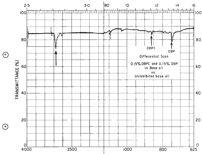
FIG. 3 Section of Differential Scan-A
