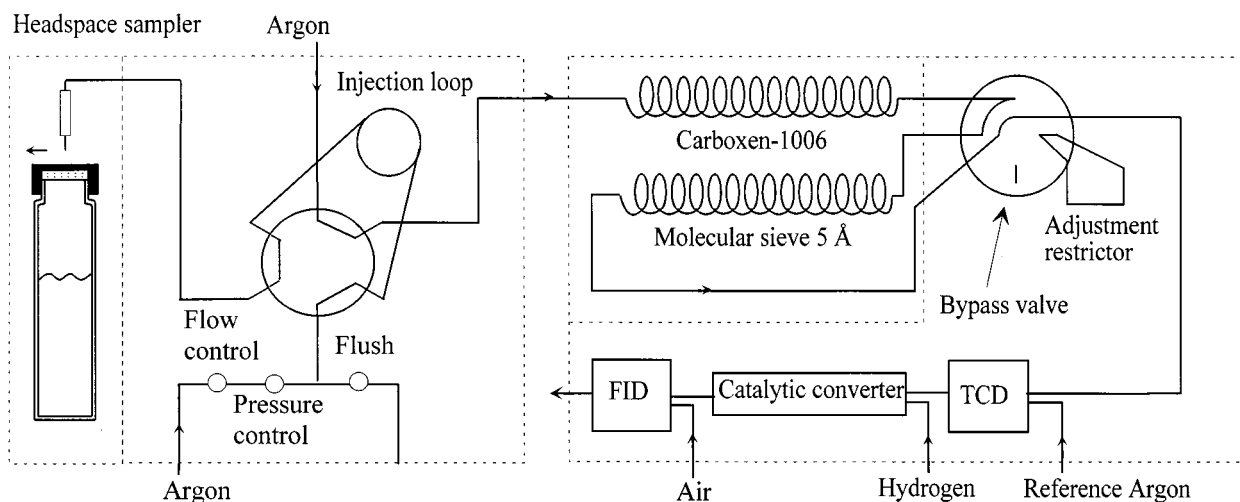
FIG. 5 Diagram of the Test Assembly (waiting mode representation).
