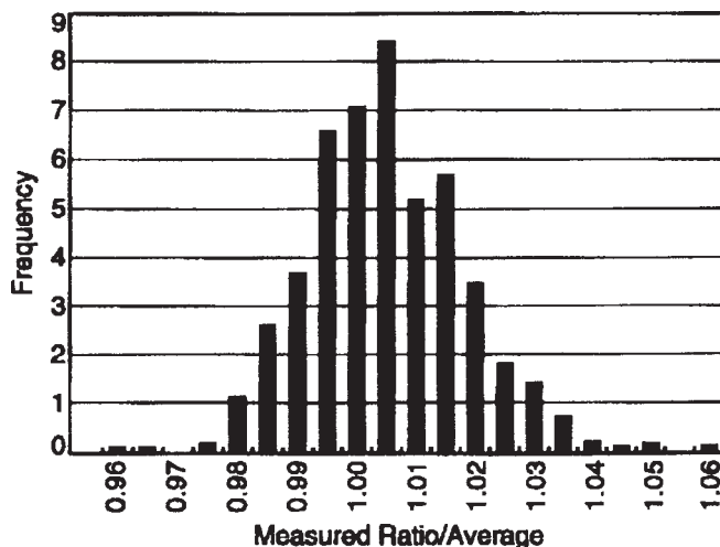
FIG. 3 Frequency Distribution of Measured Silicon/Tungsten Ratios From a Series of SPC Samples Covering >30 months
