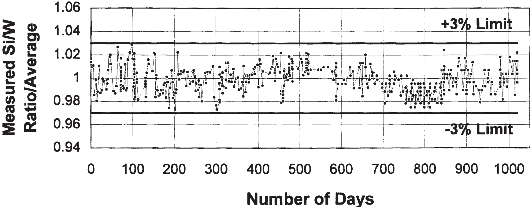
NOTE 1—Since the values were obtained from various samples with widely varying compositions, the ratios are normalized by originally measured silicon/tungsten ratios. FIG. 4 Running Plot of Measured Silicon/Tungsten Ratios Obtained in an SPC Program.
