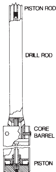
NOTE—The center section houses complex mechanical linkages. FIG. 13 Hvorslev's Thin-Wall Fixed-Piston Sampler (23)
