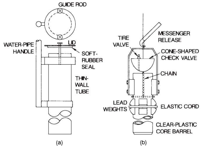
NOTE 1—(a) Modified Van-Stratten sampler. (4) (b) Milbrink's bottom sampler. (6)
