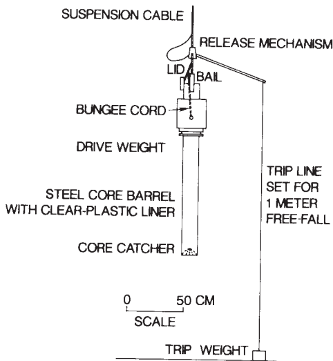
FIG. 22 SCCWRP Corer for Soft Sediments (7)
