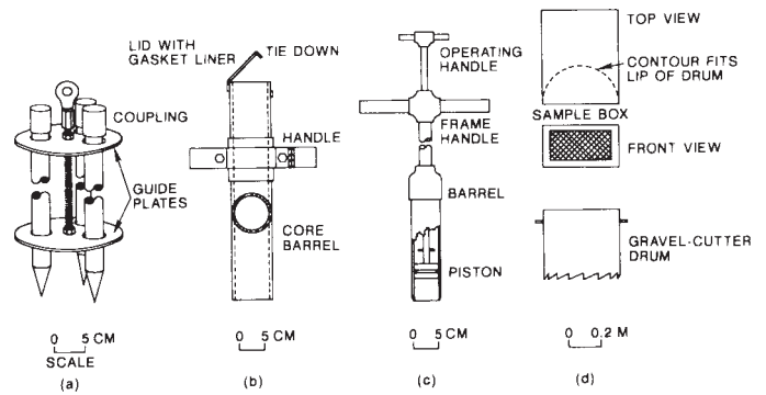
NOTE 1—(a) The cryogenic-gravel sampler, a freeze-type sampler. (20) (b) The Van Stratten, an open-barrel sampler. (4) (c) The BMH-53, a piston sampler. (21) (d) The gravel-cutting sampler. (22)
