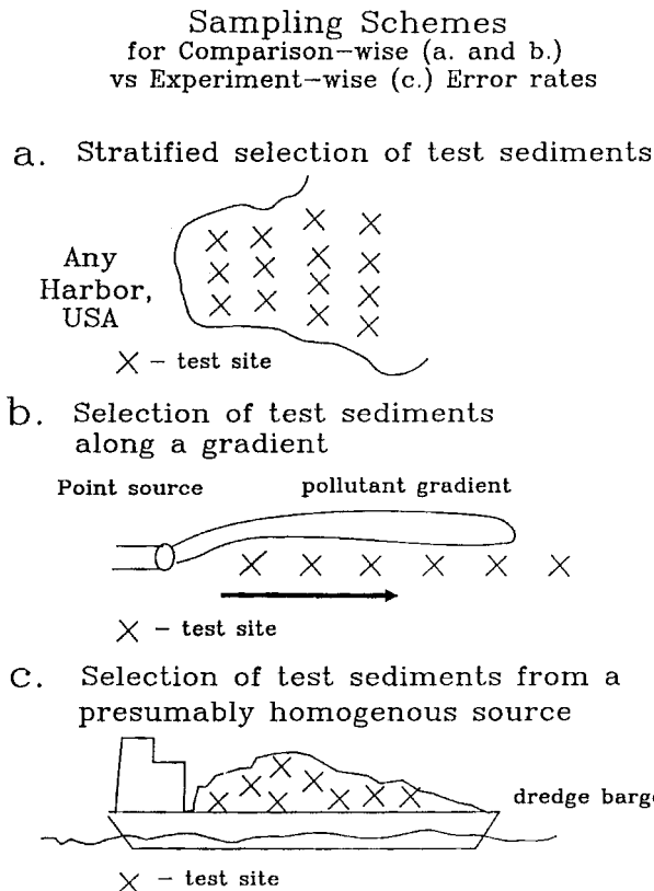
FIG. 1 Representative Sampling Schemes for Comparison-Wise Versus Experiment-Wise Error Rates
