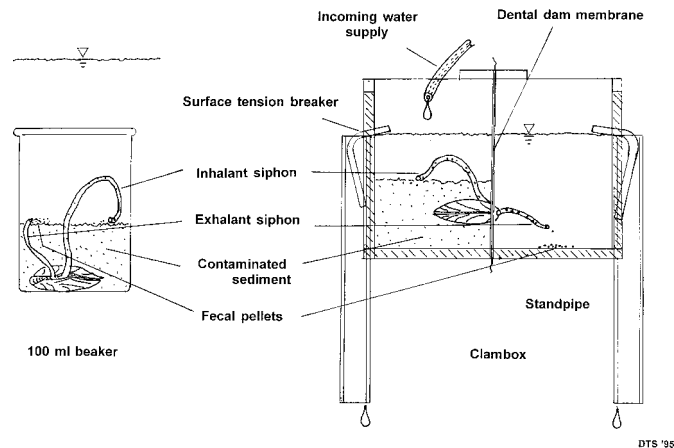
FIG. A6.1 Clam Exposure Chambers
