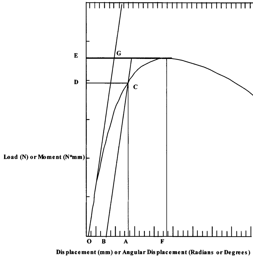
FIG. 6 Typical Load Displacement Curve
