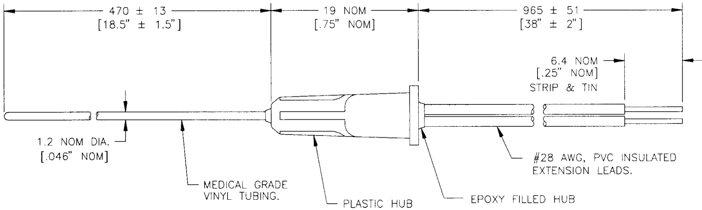
NOTE 1—Metric (English) All dimensions in millimetres unless otherwise indicated. FIG. 6 Interchangeable Sensor Enclosed in 1.2 mm Vinyl Tube
