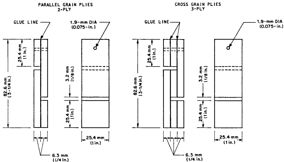
FIG. 3 Test Specimens
