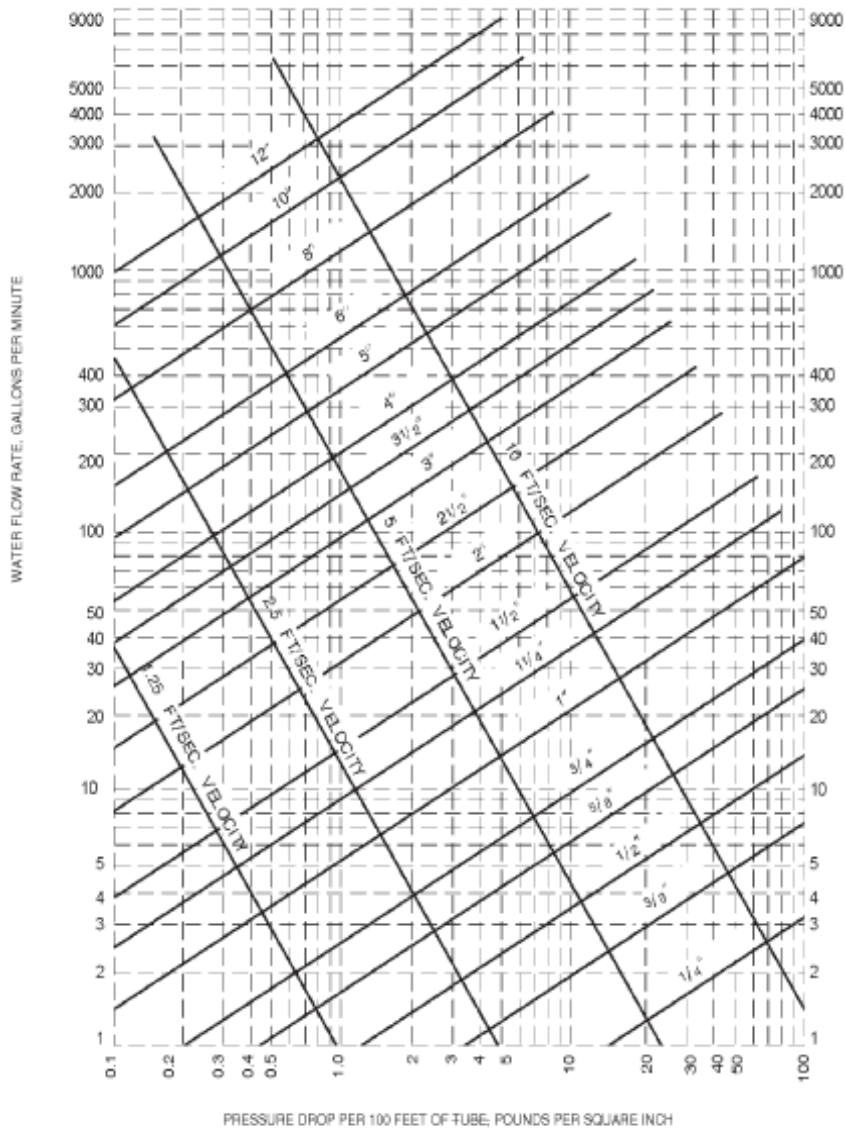
FIGURE E103.3(3) FRICION LOSS IN SMOOTH PIPE a (TYPE L, ASTM B 88 COPPER TUBING)
