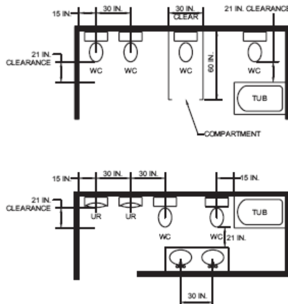
FIGURE 405.3.1 FIXTURE CLEARANCE
