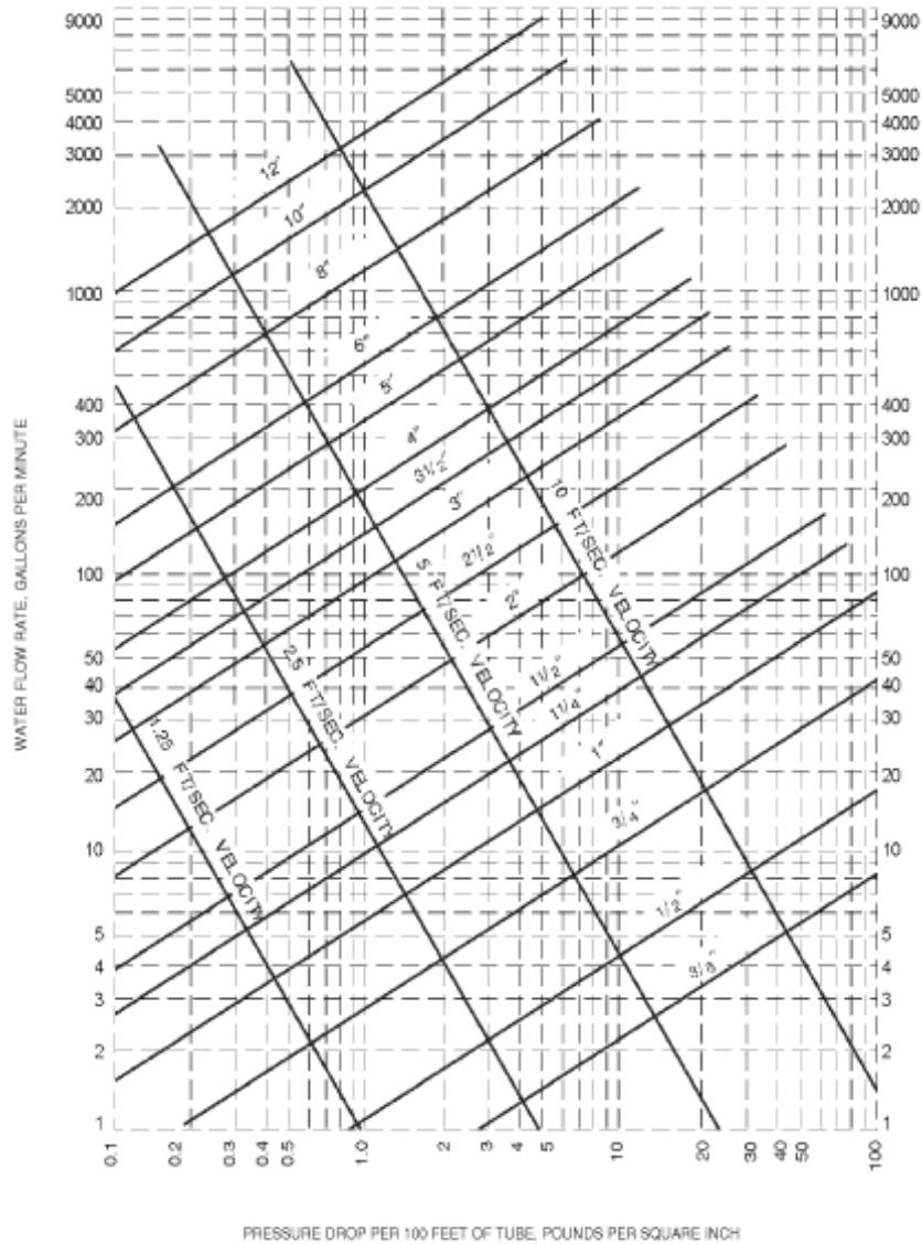
FIGURE E103.3(4) FRICTION LOSS IN SMOOTH PIPE a (TYPE M, ASTM B 88 COPPER TUBING)
