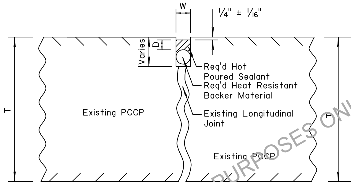
SECTION VIEW
