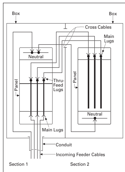
Figure 22.0-2. Through-Feed Lugs
