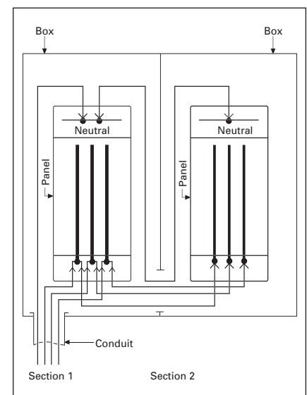
Figure 22.0-1. Sub-Feed Lugs
