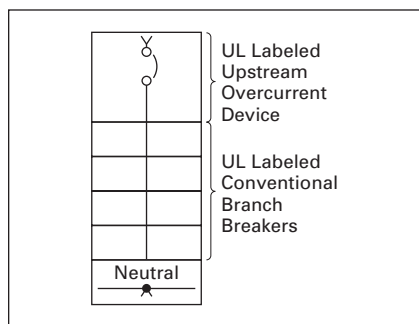
Figure 22.0-4. Main Device
