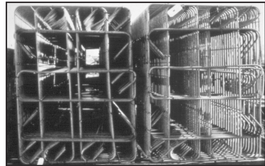
Large cages of WWR confinement reinforcement for high rise buildings.
