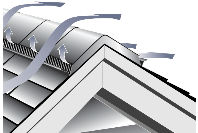
Figure 22 ShingleVent II
