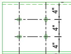
WEB PUNCHING 5/8" x 3/4" SLOTS (STANDARD)
