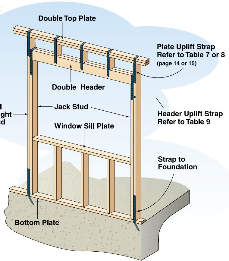
Figure 17. Studs and Headers Around Wall Openings
