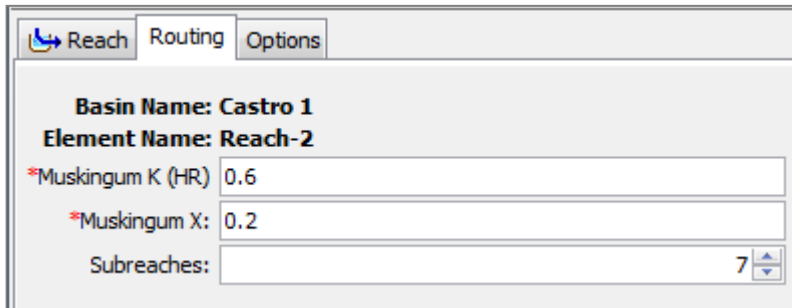
Figure 37. Muskingum data for Reach-2.
