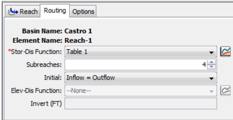
Figure 36. Modified Puls data for Reach-1.
