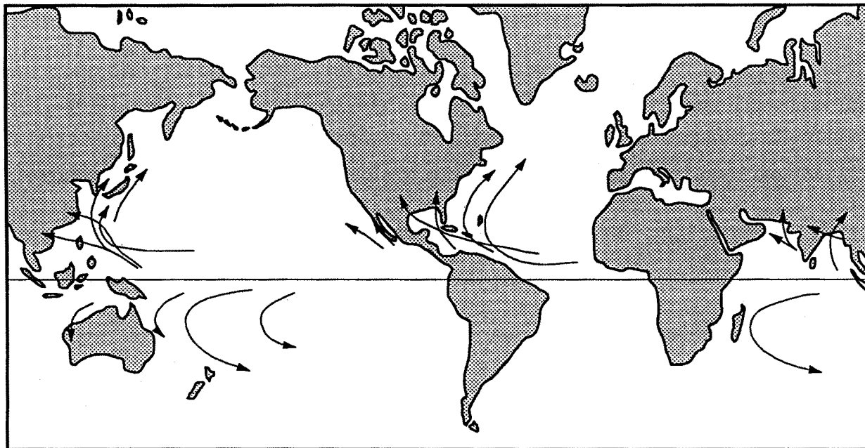
Figure IV-1-11. Worldwide tropical storm pathways (from Cole (1980))
