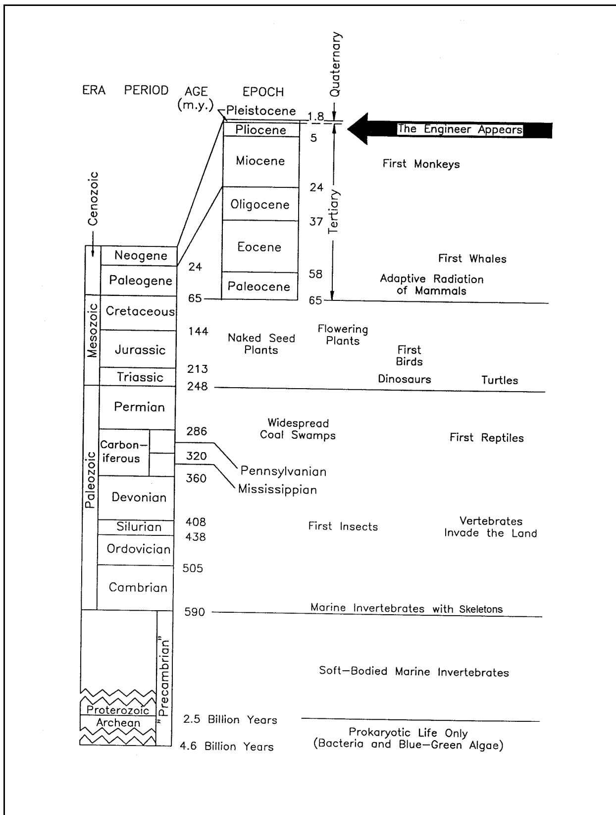
Figure IV-1-4. Geologic time scale. Chronological ages are based on radiometric dating methods (figure adapted from Stanley (1986))
