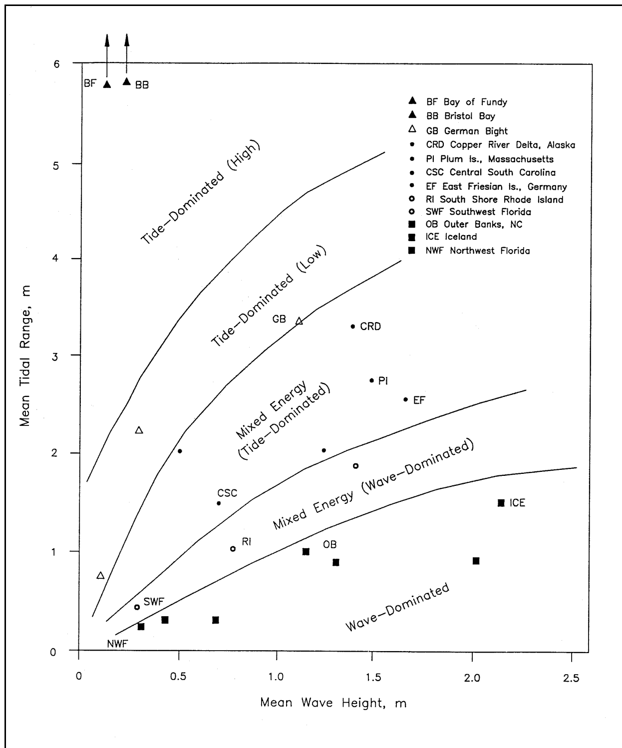
Figure IV-1-10. Energy-based classification of shorelines (from Hayes (1979))
