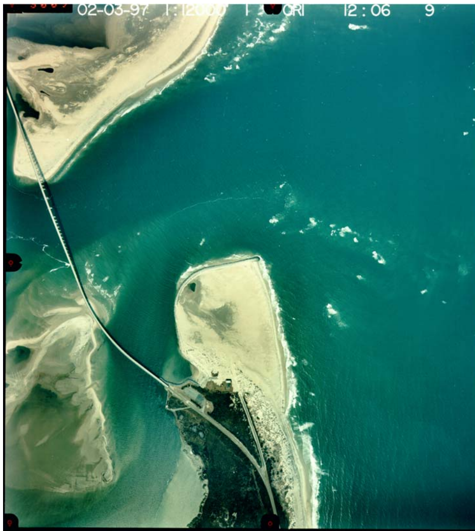
Figure V-4-30. Terminal groin, Oregon Inlet, North Carolina
