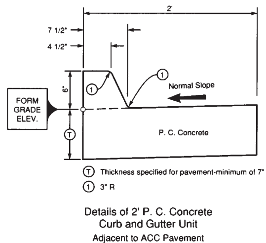
Figure 5-4. Typical curb sections
