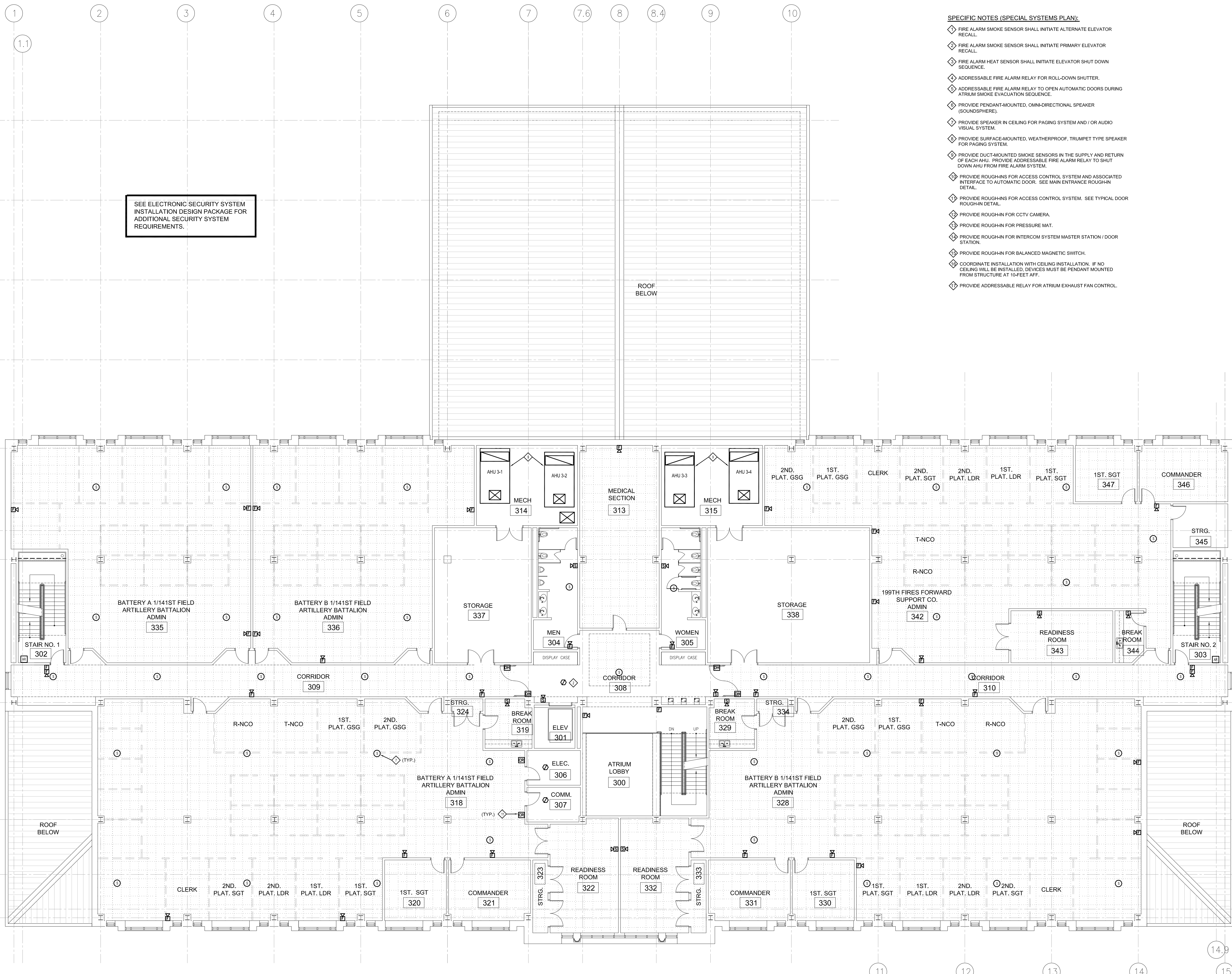
1 SPECIAL SYSTEM PLAN - THIRD FLOOR SCALE 1/8" = 1'-0"
