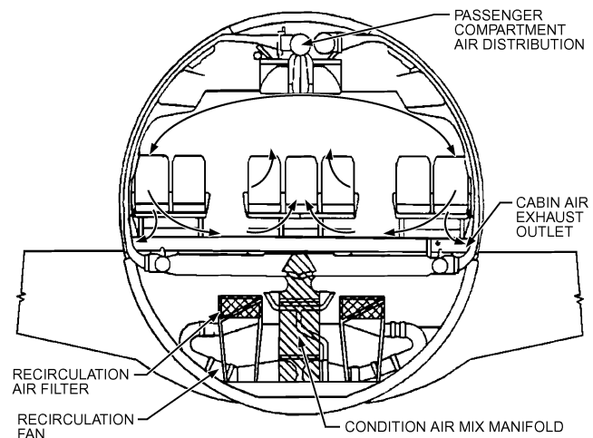
Fig. 5 Cabin Airflow Patterns (Hunt et al. 1995)
