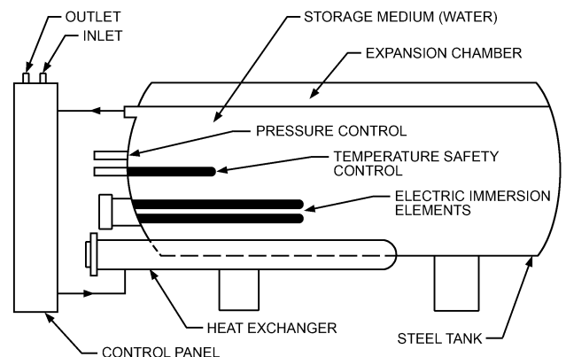
Fig. 14 Pressurized Water Heater
