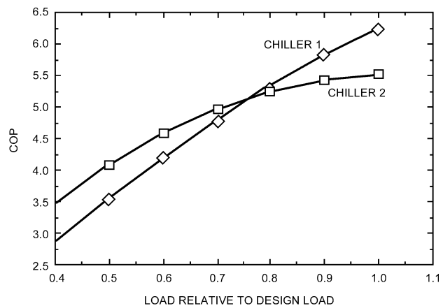
Fig. 29 Chiller COP for Two Chillers
