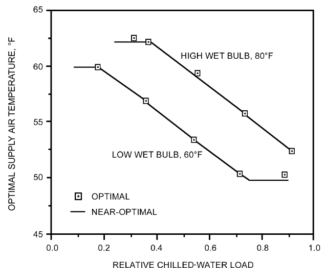
Fig. 38 Comparisons of Optimal Supply Air Temperature
