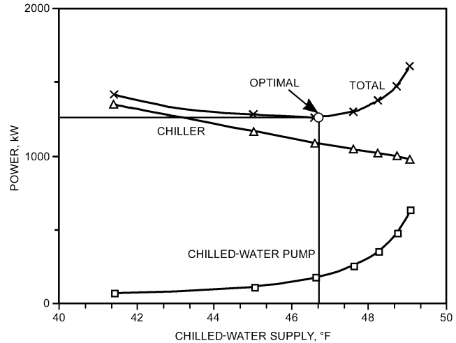
Fig. 24 Tradeoff of Chiller and Pump Power with Chilled-Water Set Point
