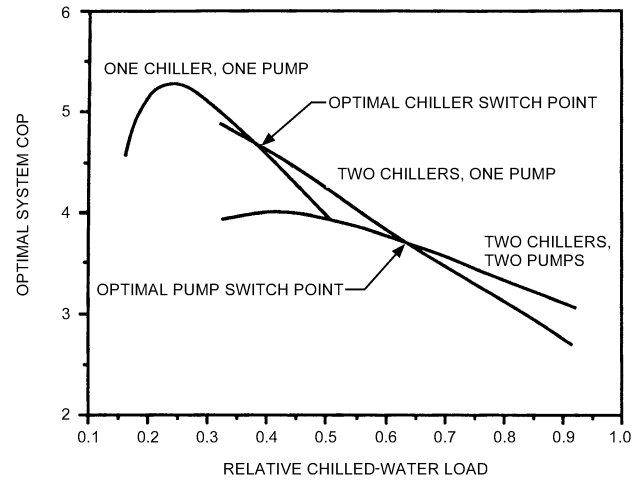
Fig. 7 Example of Effect of Chiller and Pump Sequencing on Optimal Performance
