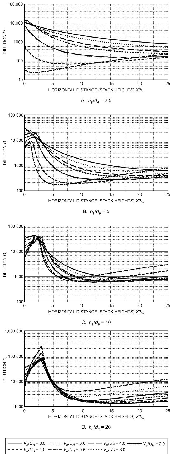
Fig. 7 Dilution Versus Distance for Uncapped Stacks
