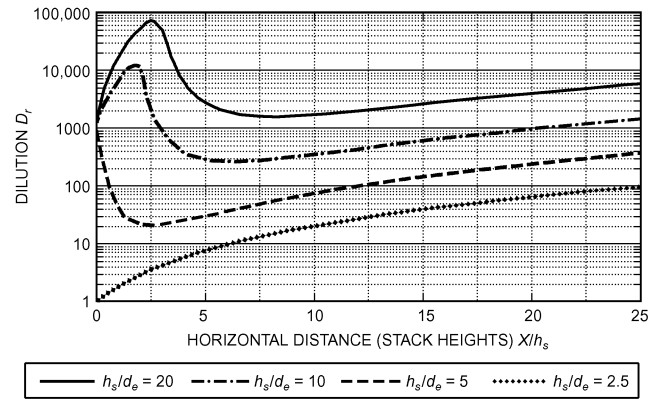
Fig. 8 Dilution Versus Distance for Capped Stack
