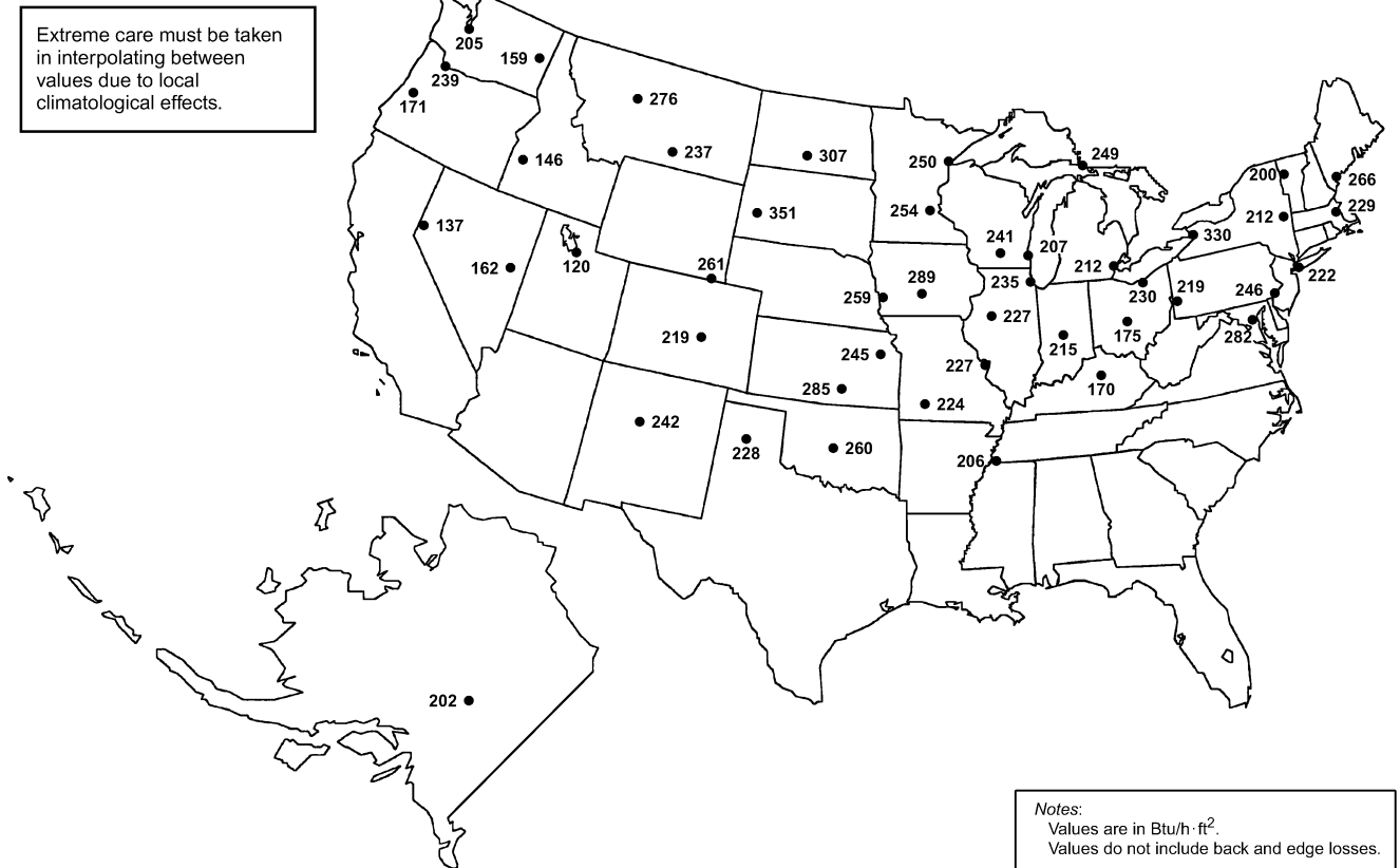
Fig. 1 Snow-Melting Surface Heat Fluxes Required to Provide Snow-Free Area Ratio of 1.0 for 99% of Time
