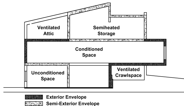
Figure 5.1 Exterior and semi-exterior building envelope.
