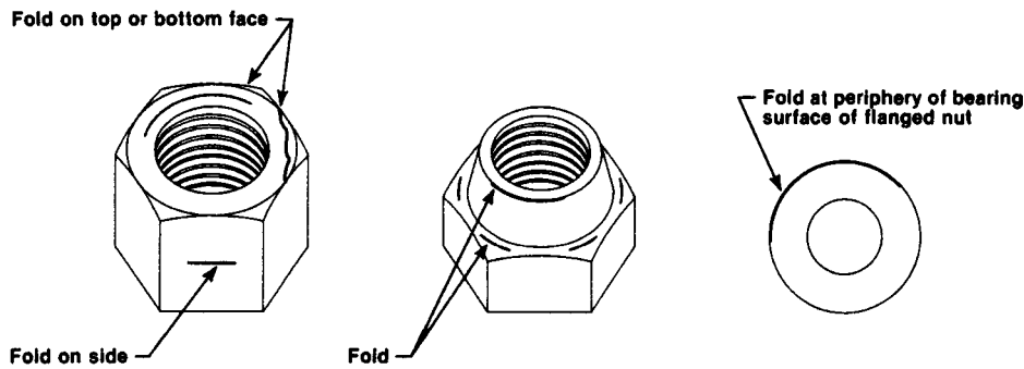
FIG. 7 Typical Folds on Surfaces of Nuts
