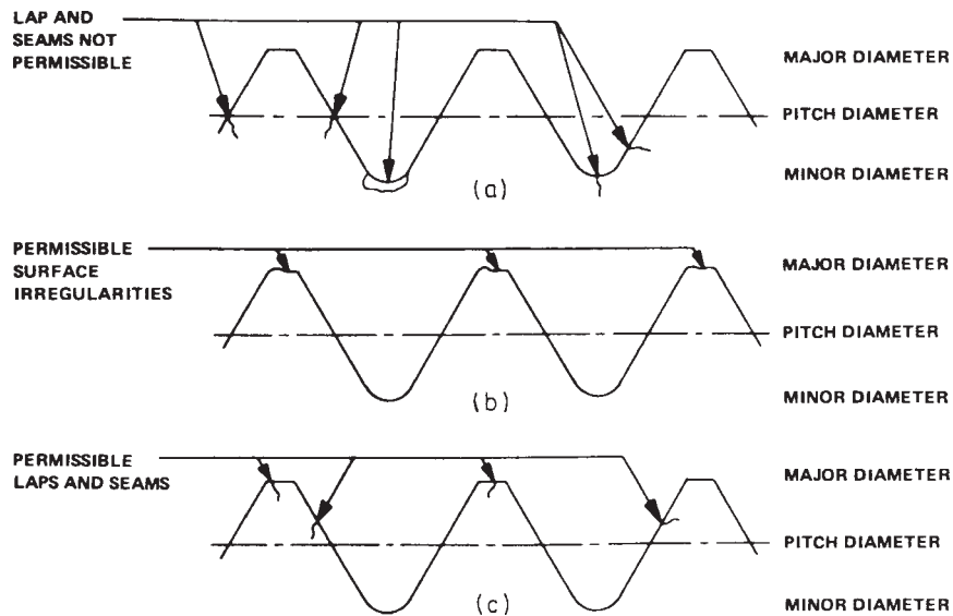
FIG. 4 Thread Discontinuities
