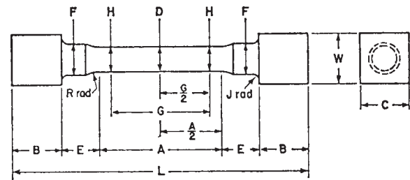
FIG. 13 Standard Tension Test Specimen for Die Castings
