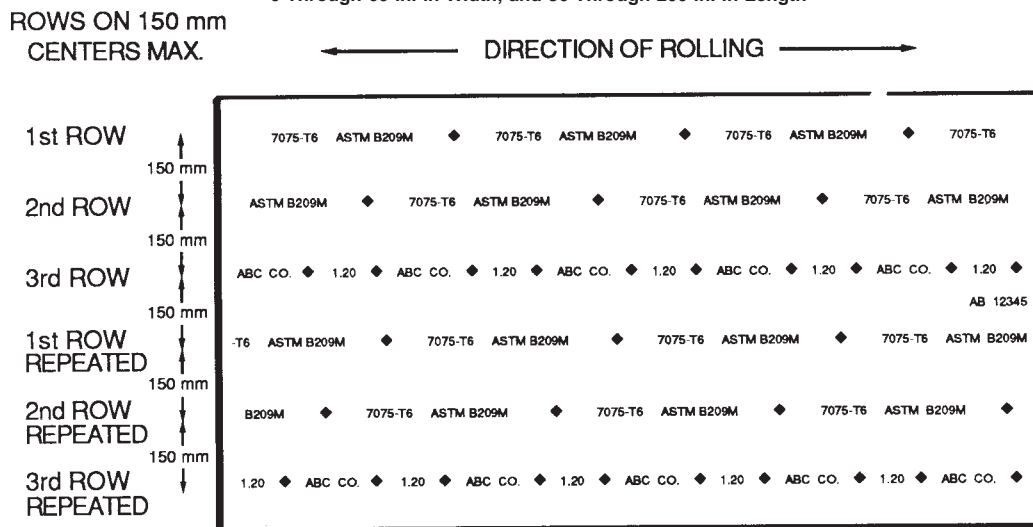
FIG 2 Continuous Marking for Plate Through 0.375 in. and Flat Sheet 0.012 in. and over (for O Temper, 0.020 in. and over) in Thickness, 6 Through 60 in. in Width, and 36 Through 200 in. in Length
