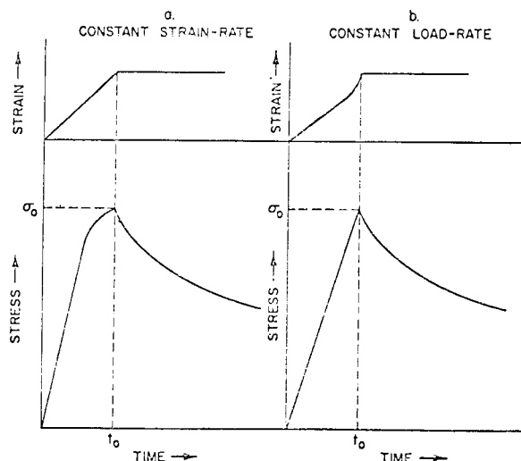
FIG. 1 Characteristic Behavior During Loading Period in a Relaxation Test
