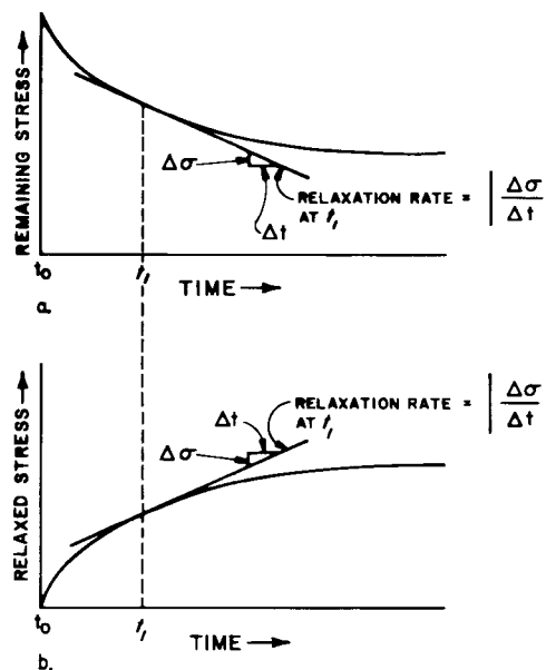
FIG. 2 Typical Relaxation Curves
