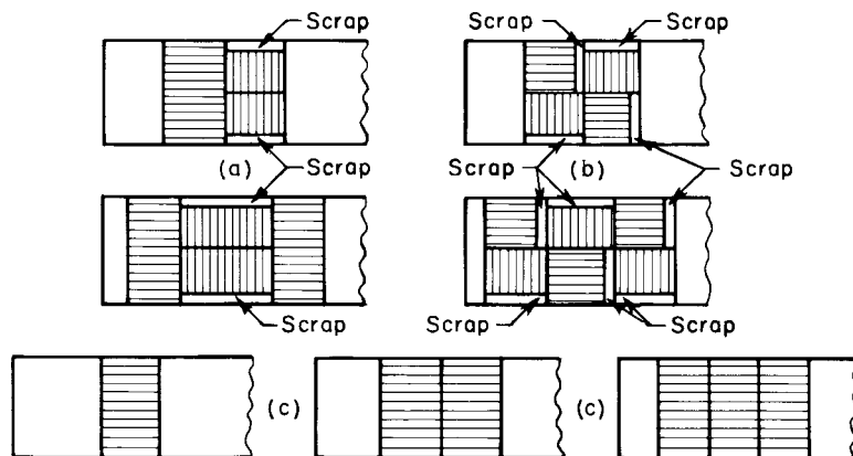
FIG. 1 Suggested Distribution of Strips to Be Cut from Sheets for Magnetic Tests
