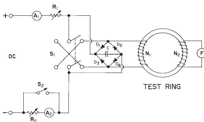
FIG. X2.1 Schematic Illustration of Arc Suppression Diode Bridge Placed in the Circuit Shown Previously in Fig. 1.
