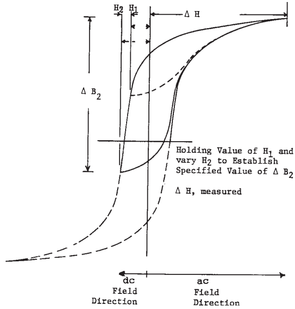
FIG. X3.8 Flux-Current Loop with Combined dc Biasing Fields, H_1 , H_2 , and Half-Wave Sine-Current Field, H_{ps} , as Used for Tests Described in 10.5
