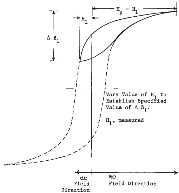
FIG. X3.6 Flux-Current Loop with Combined dc Biasing Field, H_1 , and Half-Wave Sine-Current Field, H_p , as Used for Tests Described in 10.4
