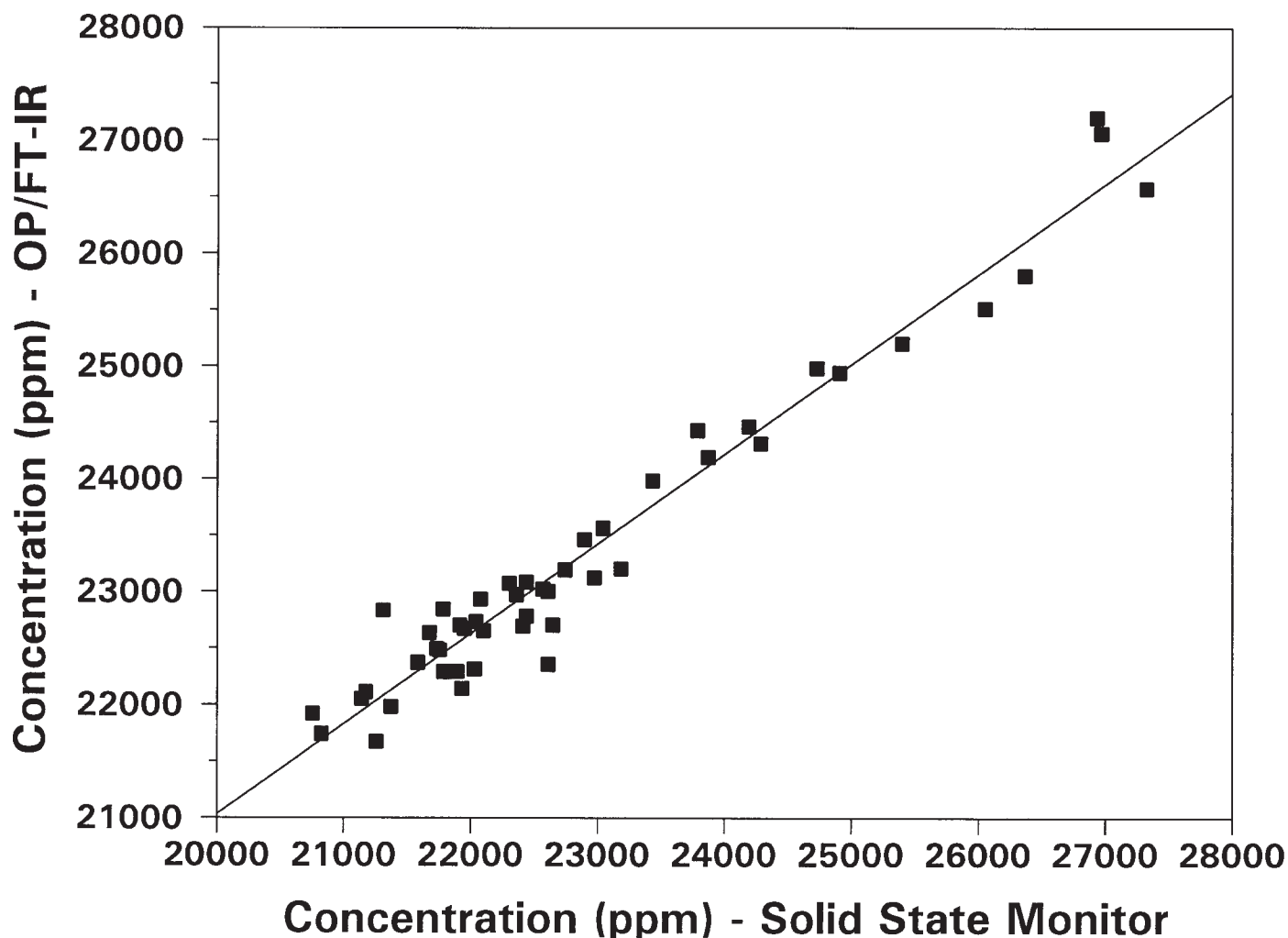
FIG. 3 Plot of the water vapor concentration over a 200-m path calculated from 0.5\text{-cm}^{-1} resolution OP/FT-IR data using a CLS analysis over the 2840\text{--}3240\text{ cm}^{-1} spectral range versus the water vapor concentration calculated from relative humidity and temperature measurements made with a solid-state point monitor.
