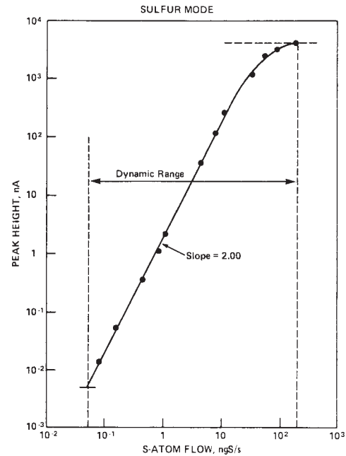
FIG. 3 Example of a Plot to Determine the Dynamic Range and Power Law of Response of an FPD in the Sulfur Mode
