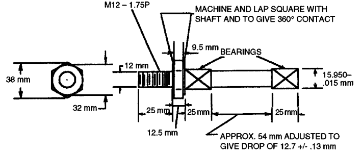
2-CAM SHAFT MEDIUM CARBON MACHINERY STEEL
