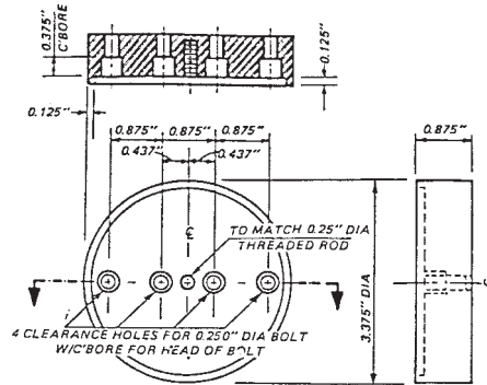
FIG. 5 Top Plate
