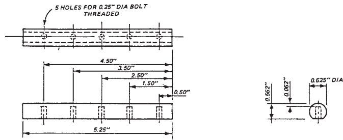
a. Rod for 6-in. (152-mm) Diameter Specimens
