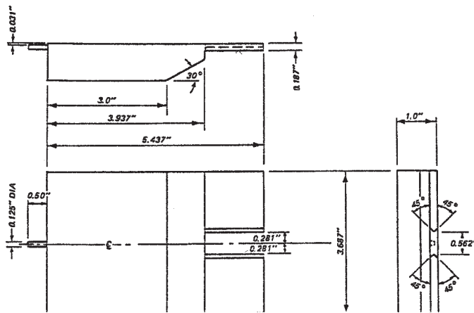
FIG. 9 Alignment Post for 4-in. (101-mm) Diameter Specimens
