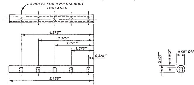
b. Rod for 4-in. (101-mm) Diameter Specimens
