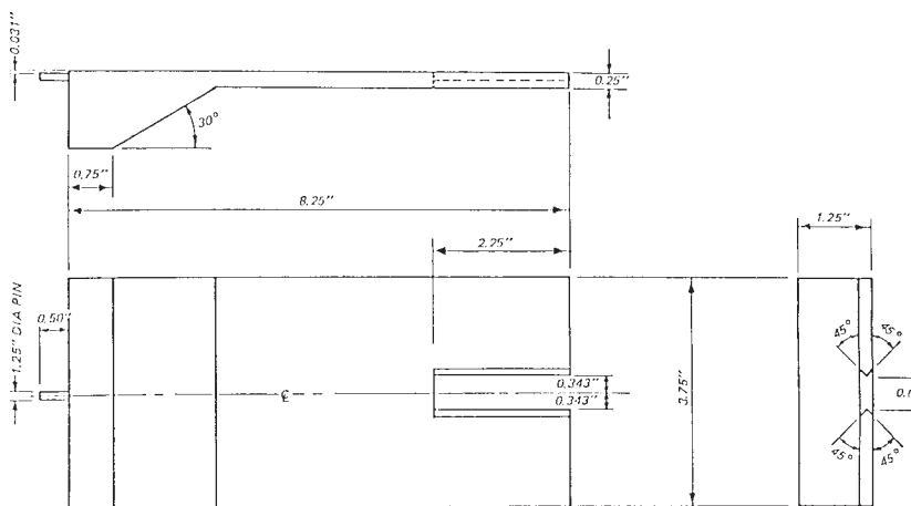
FIG. 10 Alignment Post for 6-in. (152-mm) Diameter Specimens
