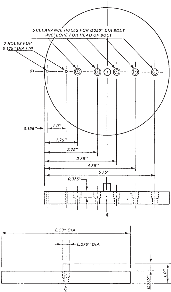
FIG. 3 Base Plate
