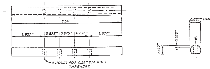
a. Rod for 6-in. (152-mm) Diameter Specimens
