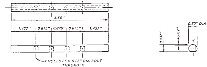
b. Rod for 4-in. (101-mm) Diameter Specimens
