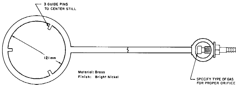
FIG. 3 Ring Burner with 4 3/4-in. (121-mm) Inside Diameter
