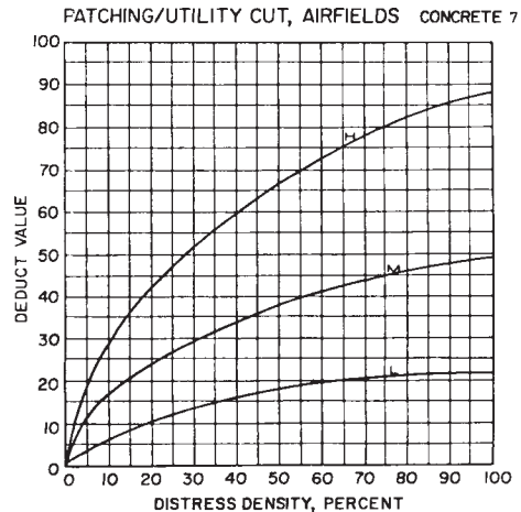
FIG. X4.7 Patching/Utility Cut
