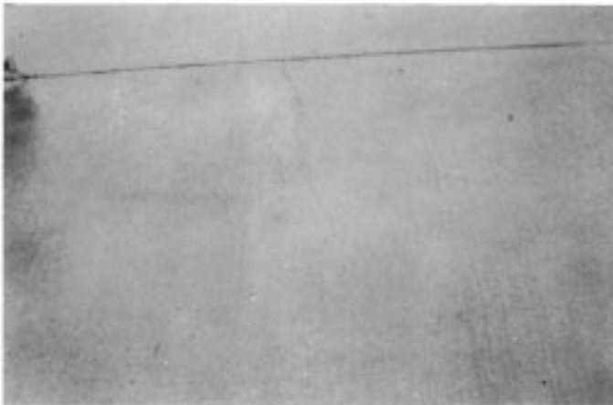
FIG. X2.61 Shrinkage Cracks
