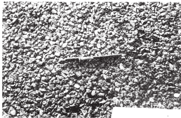
FIG. X1.63 Medium-Severity Raveling/Weathering on a Porous Friction Course Surface
