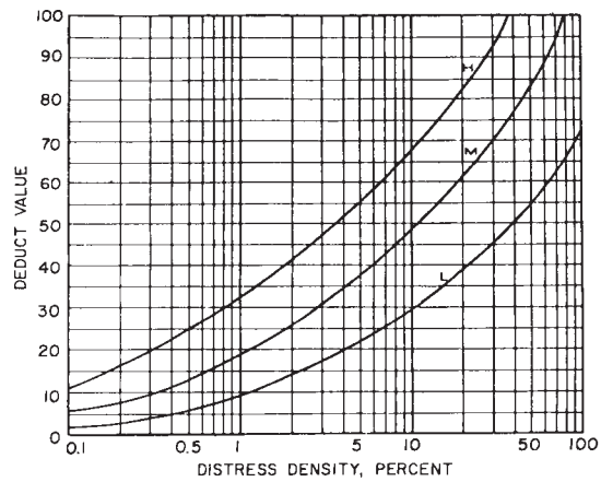
FIG. X3.4 Distress 4, Corrugation
