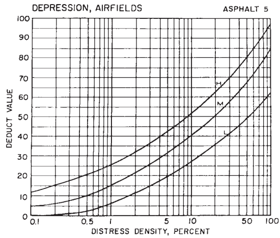
FIG. X3.5 Depression
