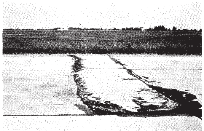
FIG. X2.2 Medium-Severity Blowup
