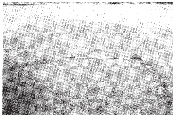
FIG. X1.25 Medium-Severity Depression (1 ½ in. (37.5 mm))
