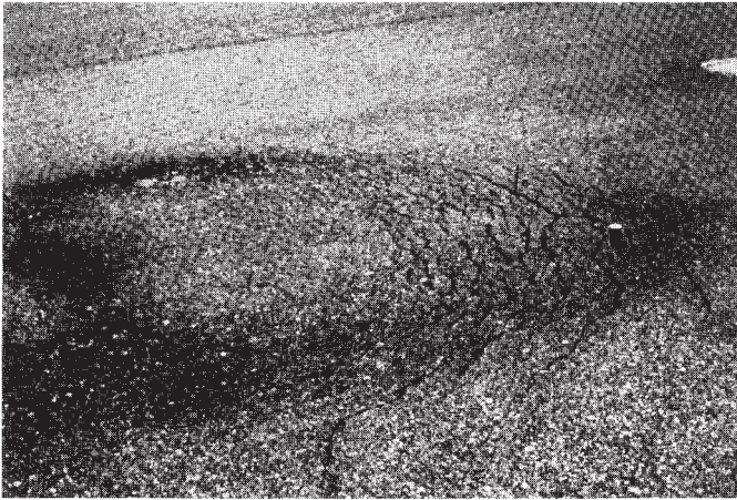
FIG. X1.73 Slippage Cracking
