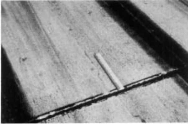
FIG. X2.59 Shrinkage Crack
