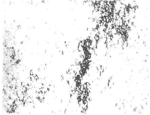
FIG. X1.57 Medium-Severity Raveling/Weathering
