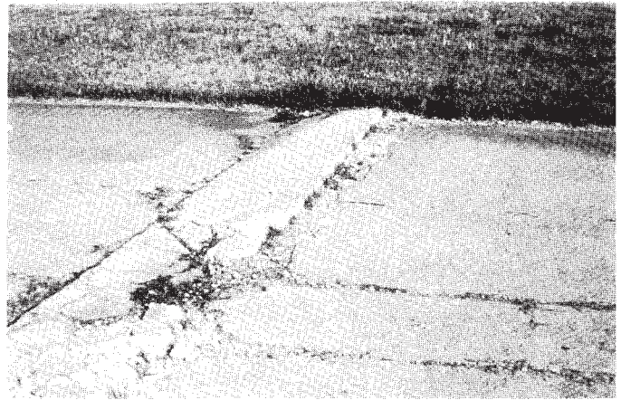
FIG. X2.3 High-Severity Blowup
