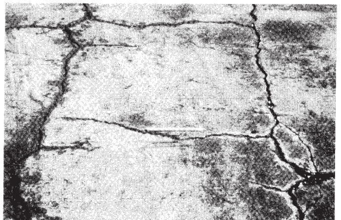
FIG. X1.16 Medium-Severity Block Cracking
