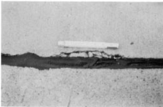
FIG. X2.64 Low-Severity Joint Spall
