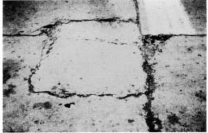
FIG. X2.37 High-Severity Patch
