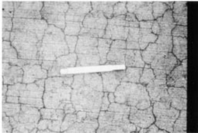
FIG. X2.44 Low-Severity Crazing
