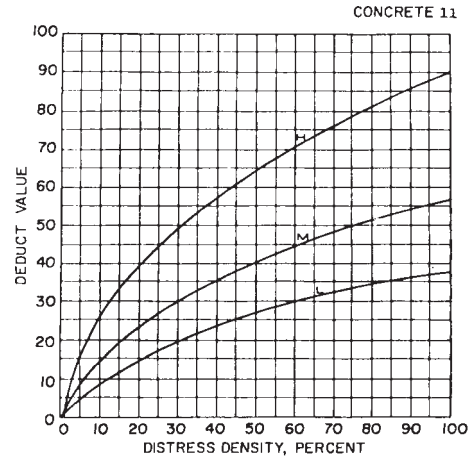
FIG. X4.11 Faulting
