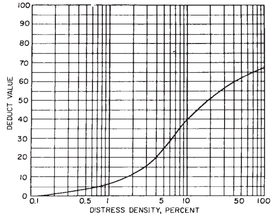
FIG. X3.2 Distress 2, Bleeding
