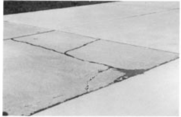
FIG. X2.56 Medium-Severity Intersecting Cracks
