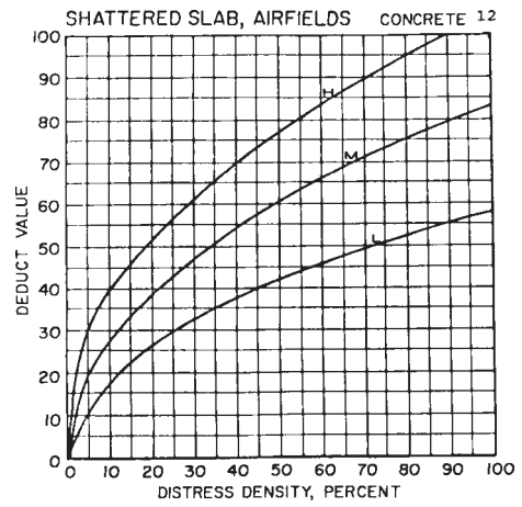
FIG. X4.12 Shattered Slab
