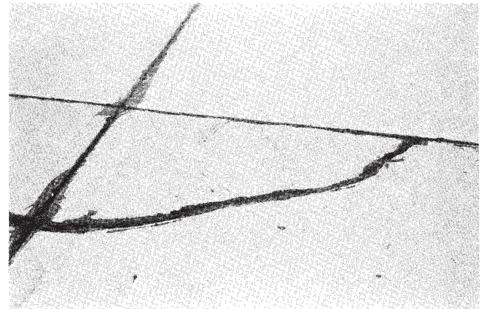
FIG. X2.6 Medium-Severity Corner Break (Area Between the Corner Break and the Joints is Lightly Cracked)
