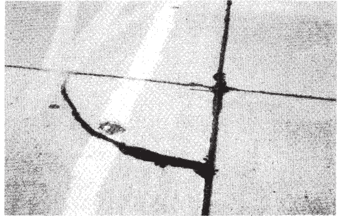
FIG. X2.5 Low-Severity Corner Break
