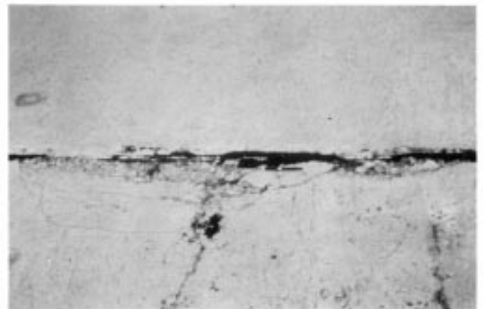
FIG. X2.67 High-Severity Joint Spall
