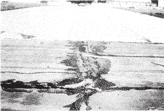
FIG. X1.78 High-Severity Swell
