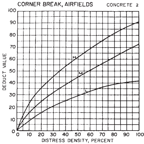
FIG. X4.2 Corner Break
