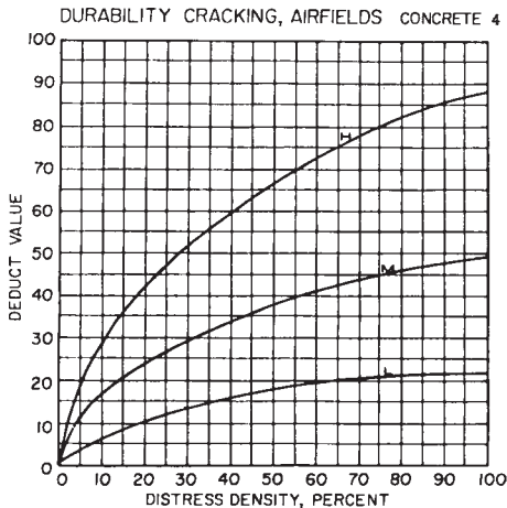
FIG. X4.4 Durability Cracking
