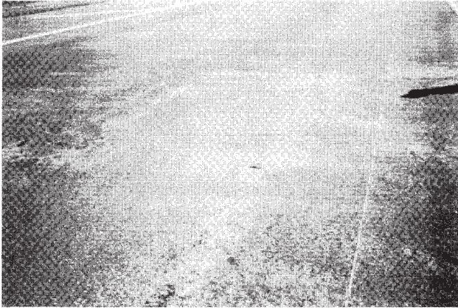
FIG. X1.22 Medium-Severity Corrugation
