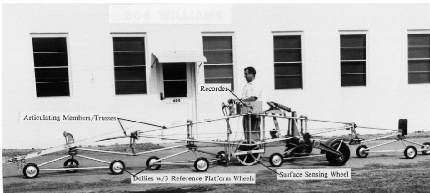
FIG. 1 Typical Profilograph
