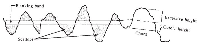
FIG. 2 Surface Record
