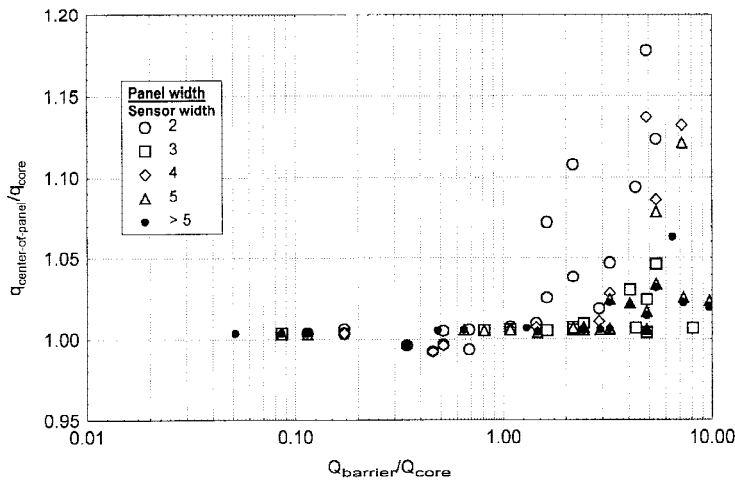
FIG. X1.1 Effect of Panel Construction on Measurement Requirements Based on the Parametric Analysis Summarized in Table X1.1
