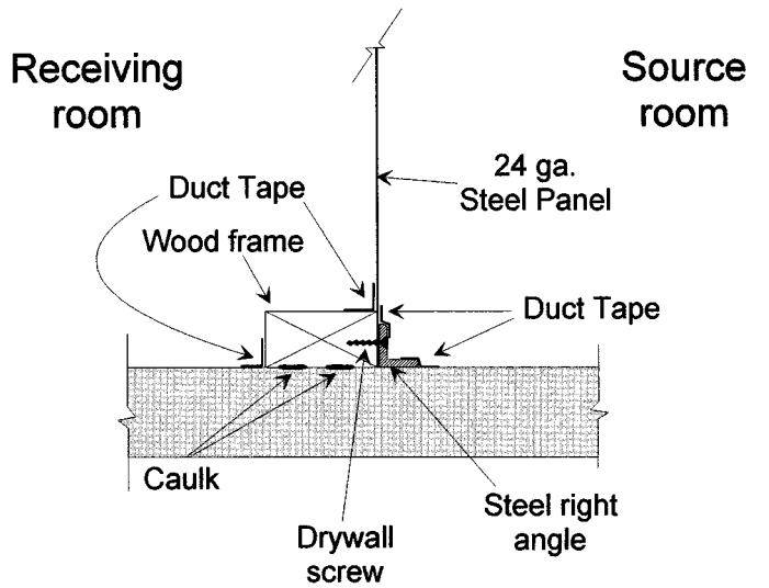
FIG. 4 Installation of Reference Specimen Showing Caulking of Wood Frame and the Taping of the Specimen Joints and Perimeter on Both Sides
