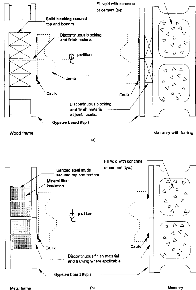
FIG. 6 Typical Wall/Jamb Details
