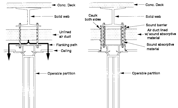
(a) Sound flanking paths
