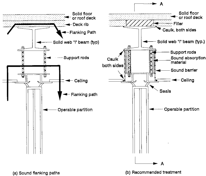
(a) Sound flanking paths
