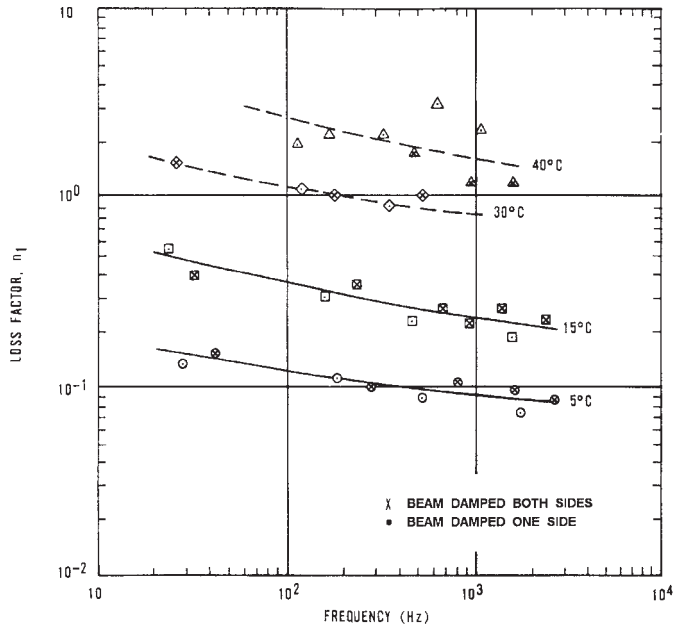
FIG. 9 Damping Material Loss Factor Versus Frequency for Various Temperatures
