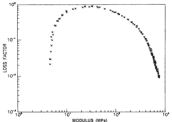
FIG. X2.1 Wicket Plot
