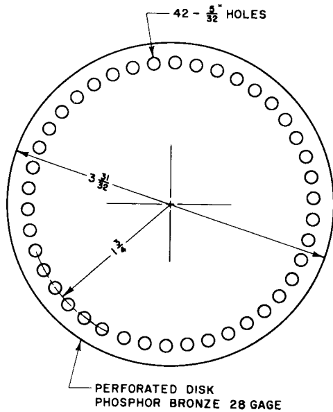
FIG. 5 Phosphor-Bronze Disk
