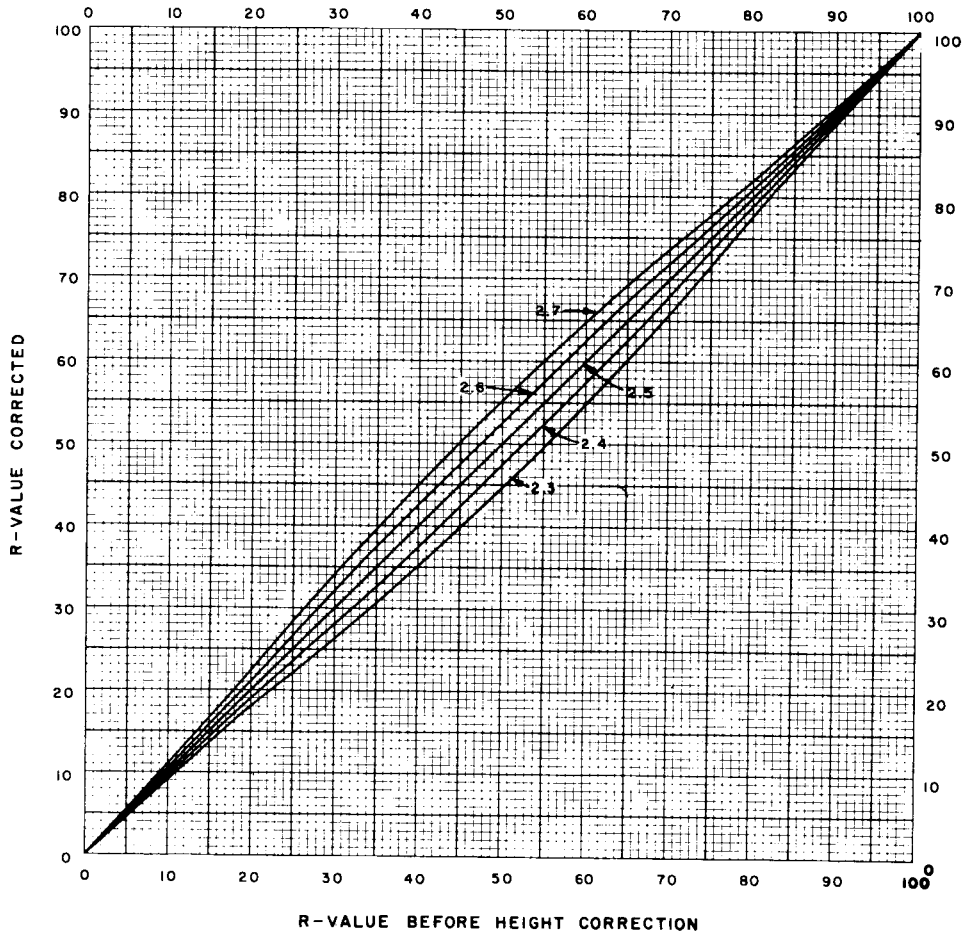
R-VALUE BEFORE HEIGHT CORRECTION FIG. 9 Height-Correction Chart
