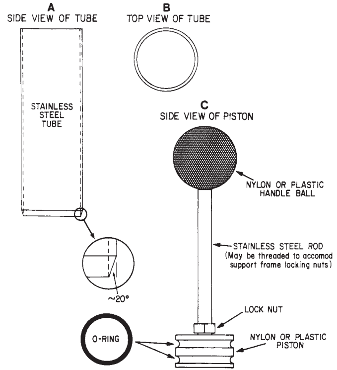
FIG. 1 Thin-Walled Piston Sampler
