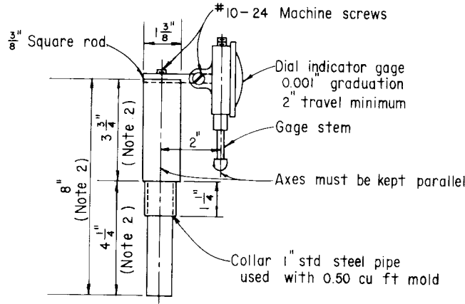
(c) Holder for Dial Indicator Gage
