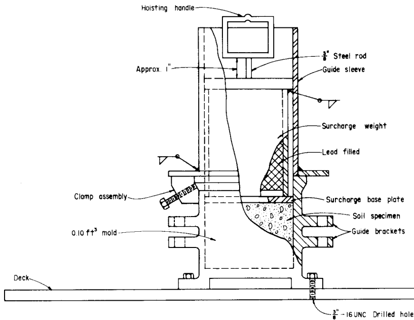
FIG. 1 Schematic Drawing of a Typical Mold Assembly
