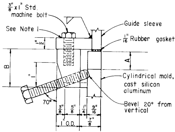
(a) Typical Clamp Assembly for Guide Sleeve for Guided Surcharge Weights.
