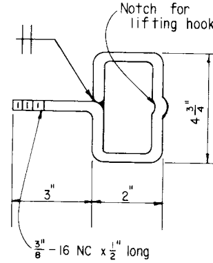
(b) Surcharge Base Plate Handle (1 Required)
