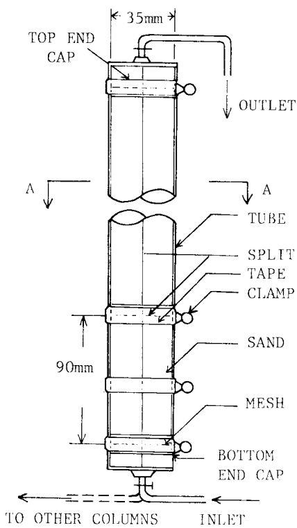
FIG. 1 Specimen Mold
