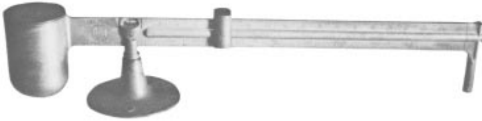
FIG. 1 Mud Balance
